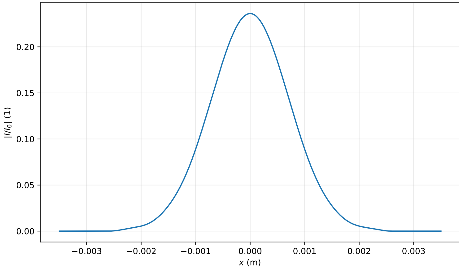
Intensity profile I(x, y = 0, z = 3.821m)/I_0 , P_{in}=0.1P_{cr} , artificial time
